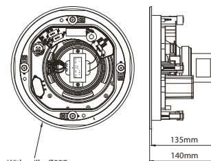
With grille: Ø257mm Without grille: Ø247mm Hole Cut: Ø220mm
