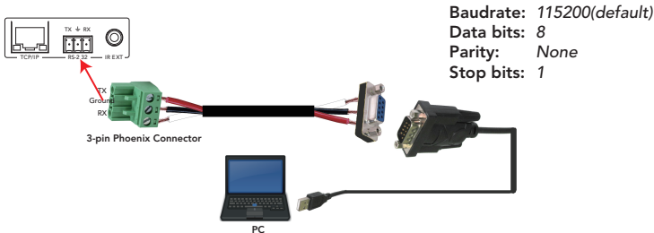
Figure 1: 3-pin phoenix connector to USB
