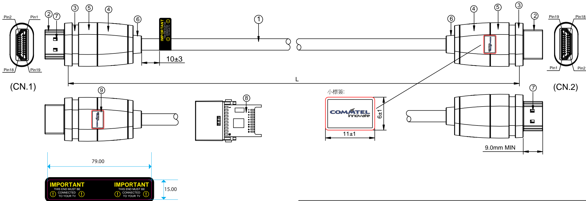
(A).Wire Pin Assignment and Wire Description.
