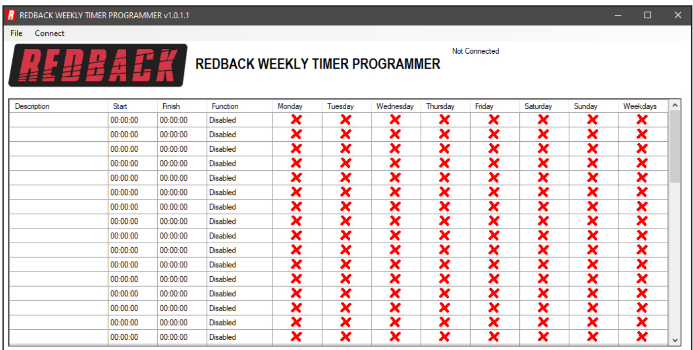
Fig 1.0 Programming Screen
