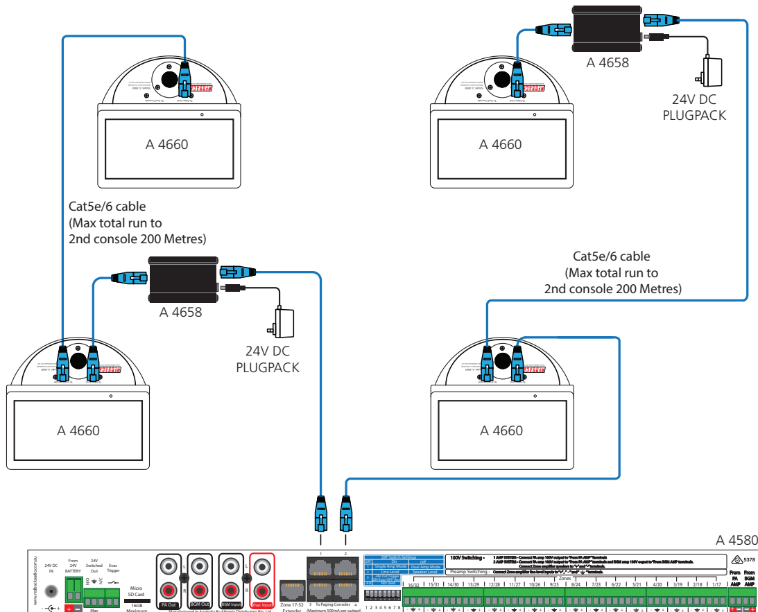
Fig 1. Connecting A 4658 power injectors into the Cat5e/6 cable run.
