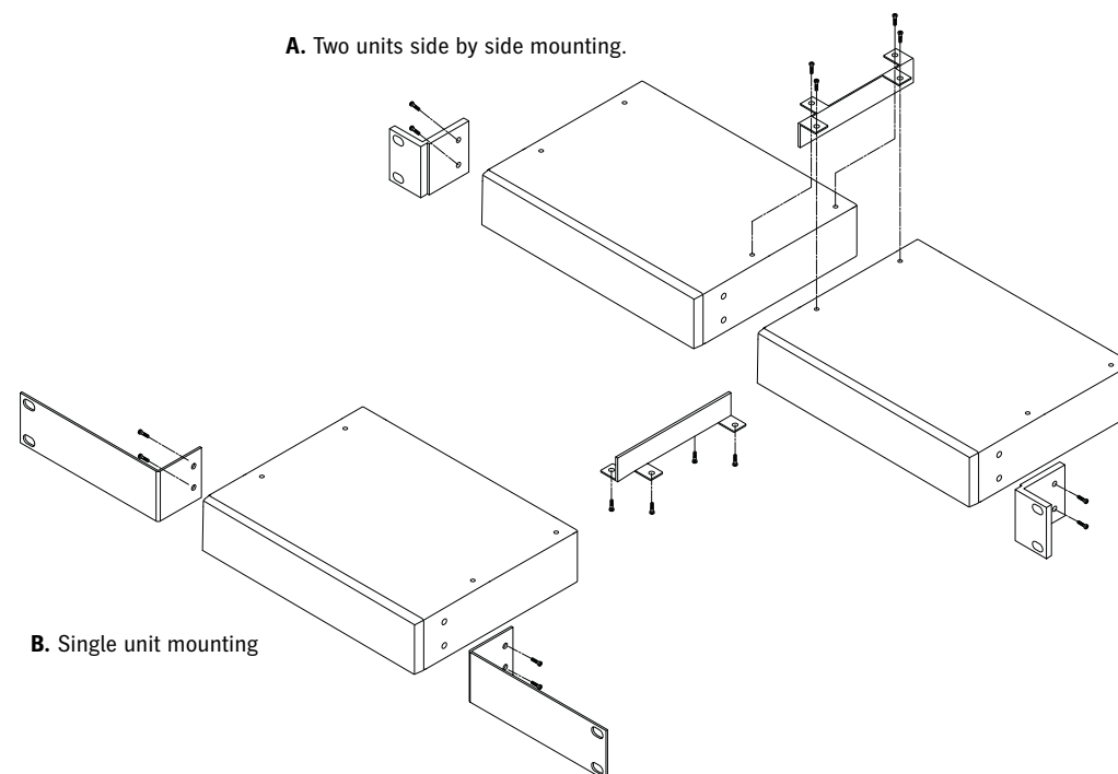
Fig. 11: Mounting C 7281A & C 7282A In 19" Racking
