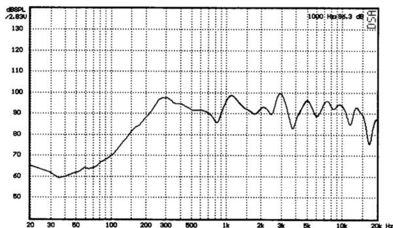
Frequency Response
